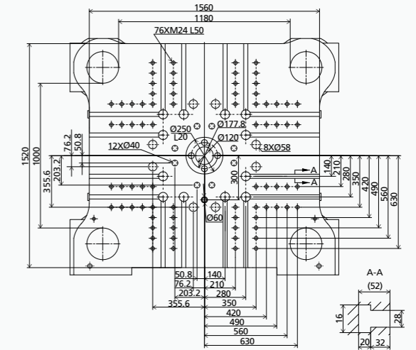
MOVABLE PLATEN
