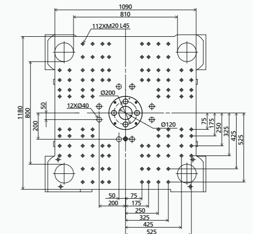
MOVABLE PLATEN
